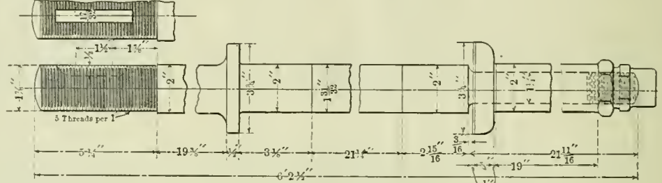
DETAIL OF VALVE STEM
